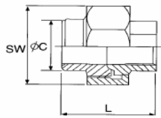
. Welded-threaded union Ref. 2028
