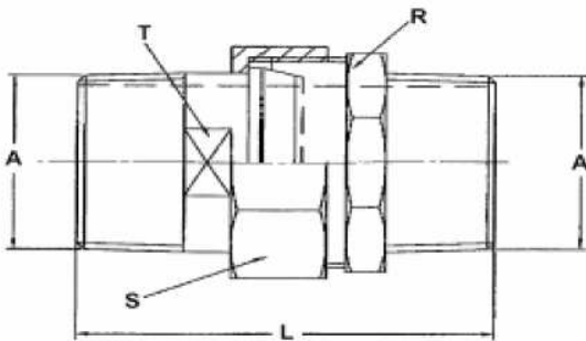
Union male/male Ref. 2064
