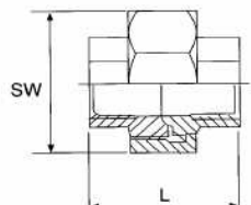
· Union female/female Ref. 2025
