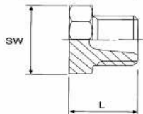
· Hexagon plug Ref. 2022 or 2023 (plain)
