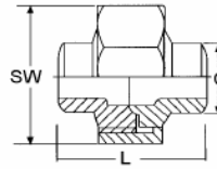
. Welded union Ref. 2029
