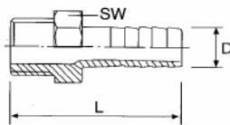
. Hose nozzle Ref. 2035
