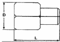
. Reduced nipple female/male Ref. 2033
