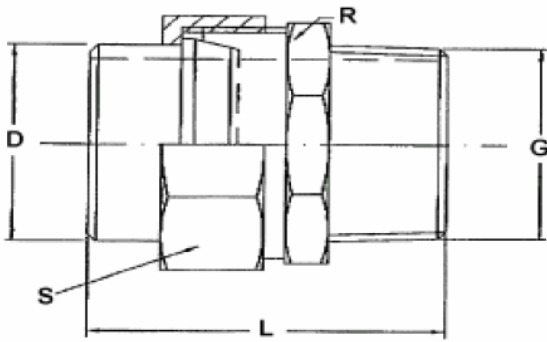
Welded/male union Ref. 2067
