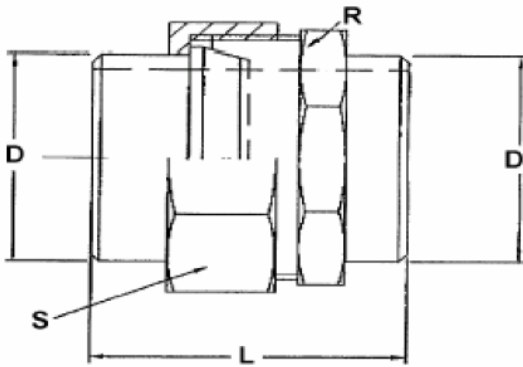
BW/BW union Ref. 2069
